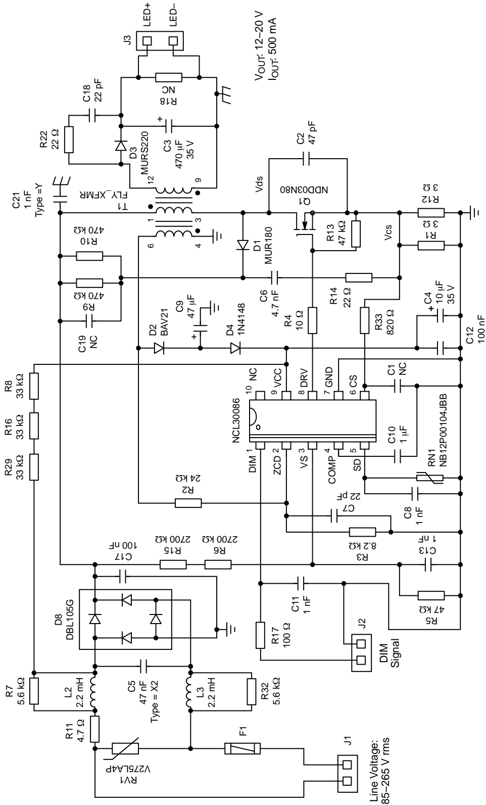
Figure 7. Application Schematic
