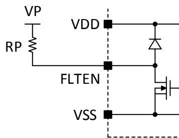
Figure 21. Fault Connection
