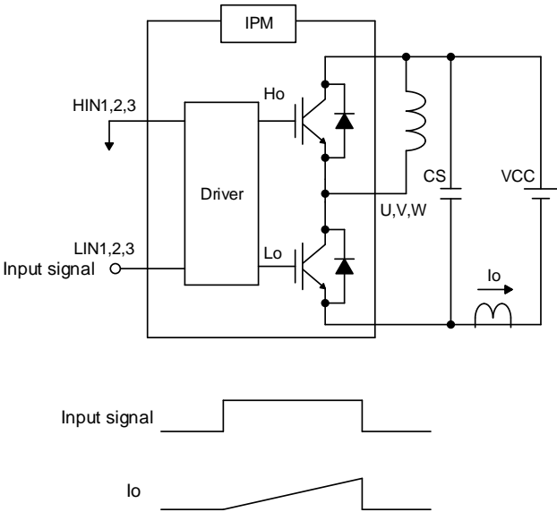
Figure 6. R.B.SOA circuit
