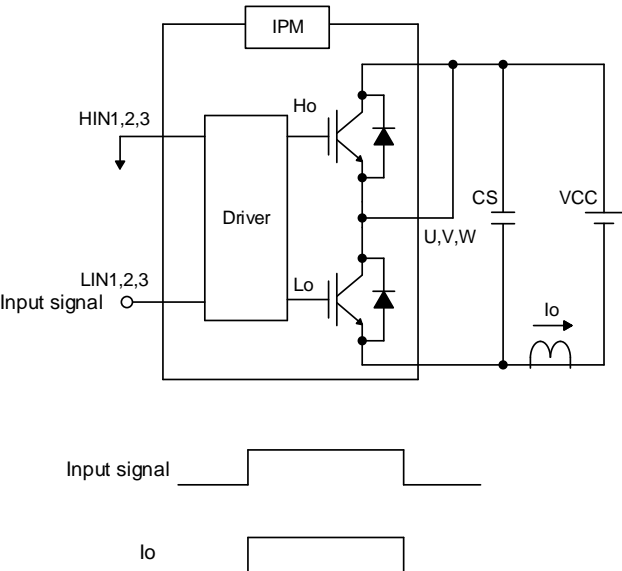
Figure 7. S.C.SOA circuit
