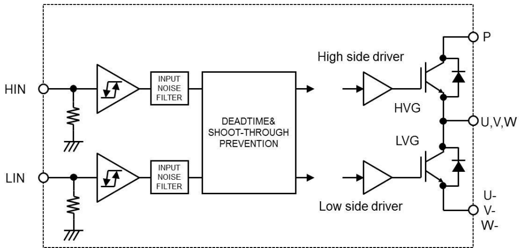
Figure 14. Cross Input Conduction Prevention
