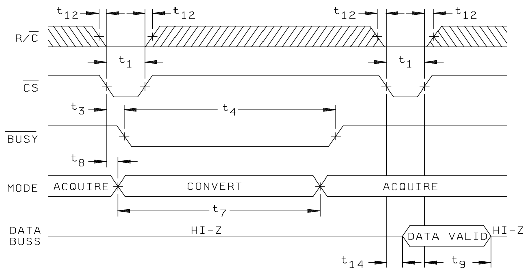
USING \overline{CS} TO CONTROL CONVERSION AND READ TIMING
