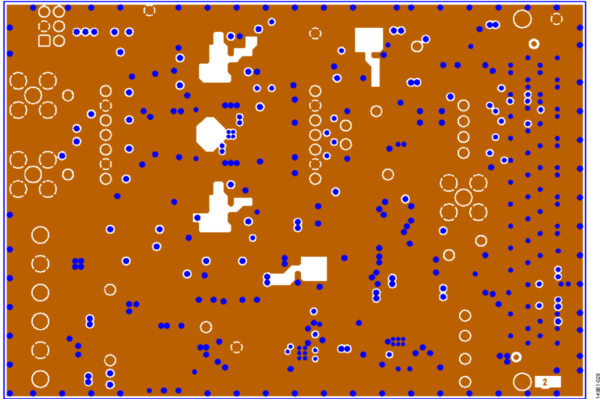
Figure 31. ADC Evaluation Board, Layer 2
