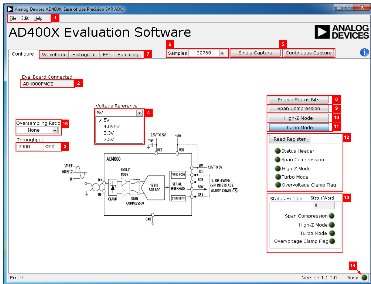
Figure 18. Setup Screen
