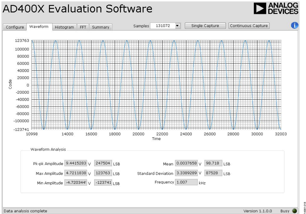
Figure 21. Waveform Tab
