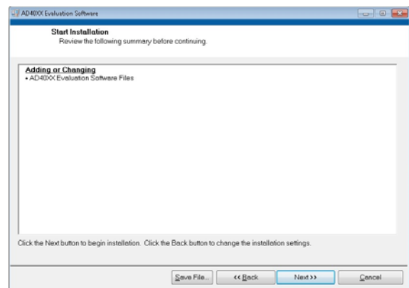
Figure 6. Start Installation
