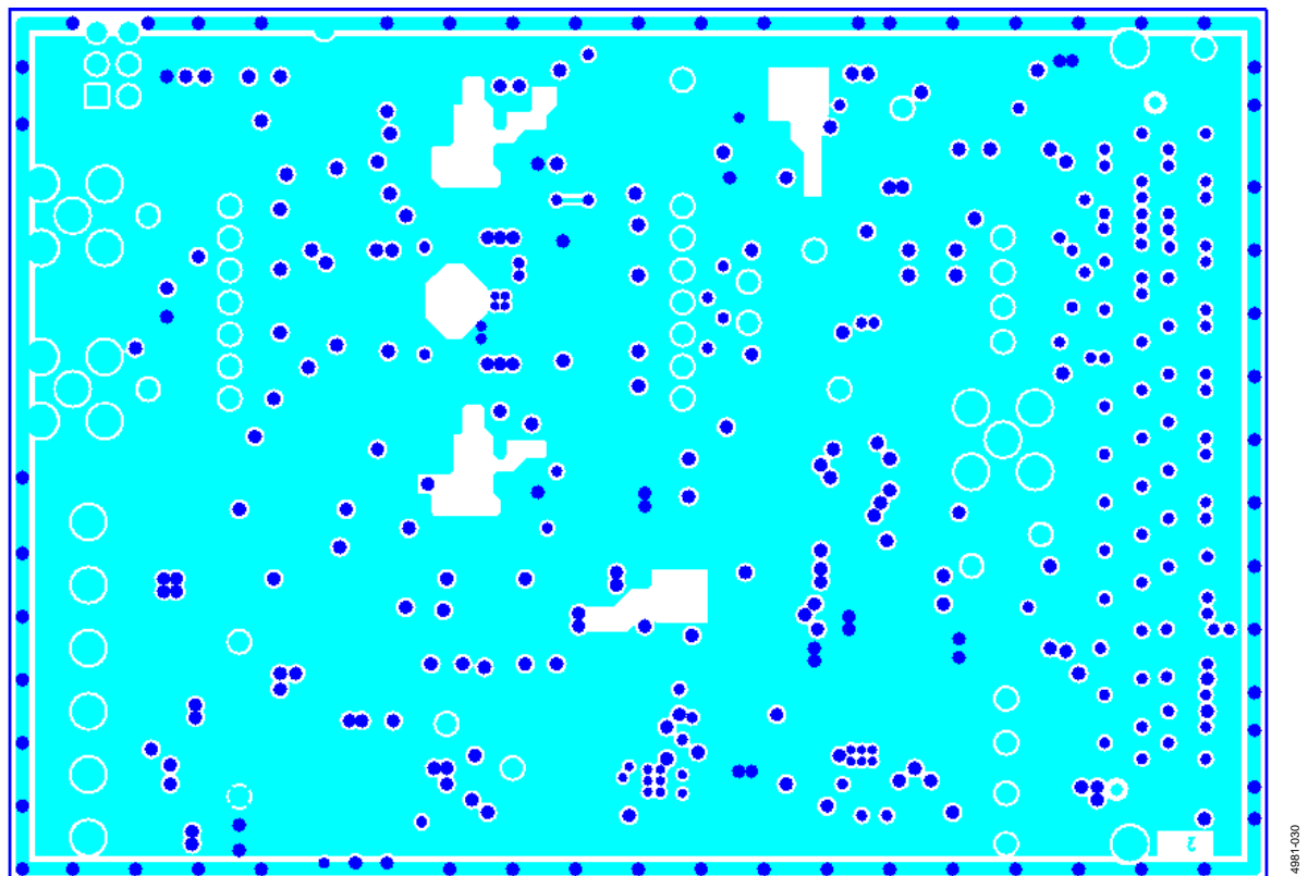
Figure 32. ADC Evaluation Board, Layer 3
