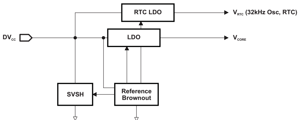
Figure 1. PMM Block Diagram
