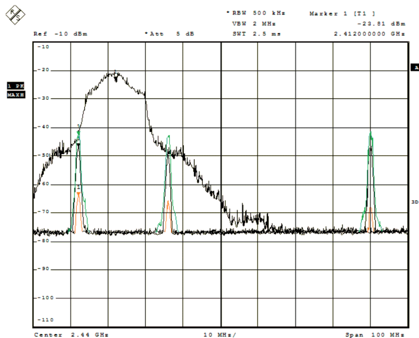
Figure 8. Spectrum for Wi-Fi Channel 1 versus Beacon Advertisement Channels
