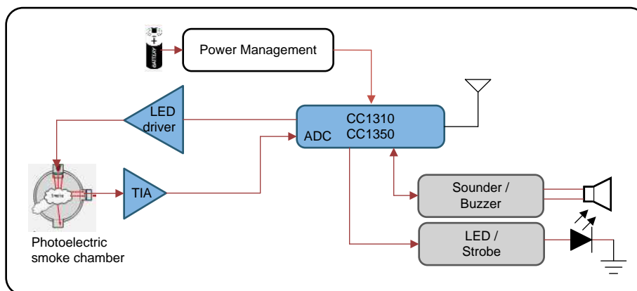
Figure 1. Photoelectric Smoke Alarm System Block Diagram
