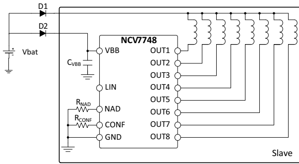
Figure 2. Device Setup
