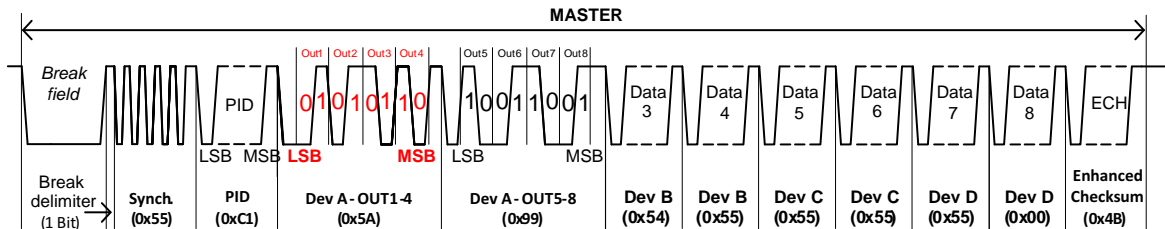
Figure 3. LIN Output Control Frame
