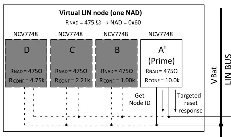
Figure 1. Virtual LIN Node
