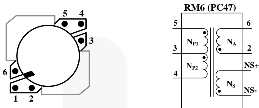
Figure 11. Transformer Specifications & Construction
