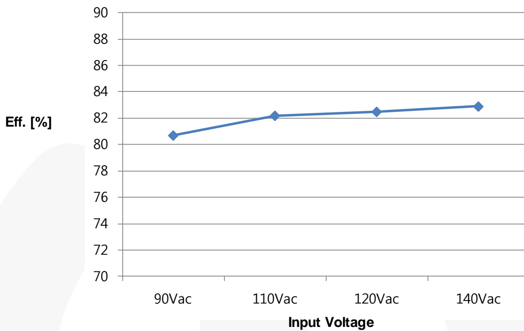
Figure 22. Power Efficiency (Input Voltage vs. Efficiency)
