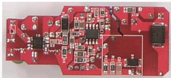
Figure 3. Bottom View of Evaluation Board
