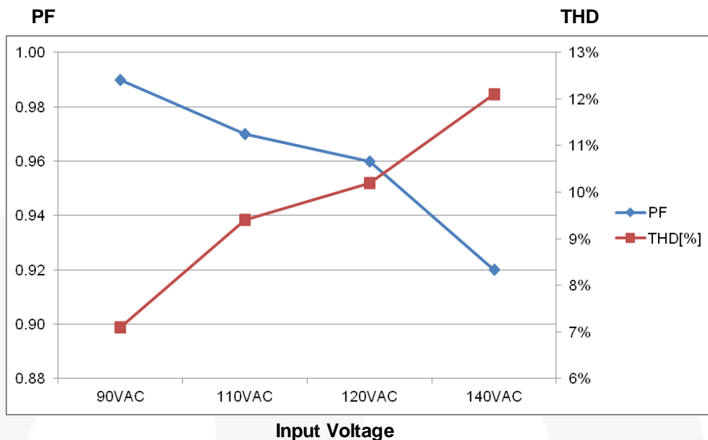
Figure 23. Power Factor & Total Harmonic Distortion (50Hz)
