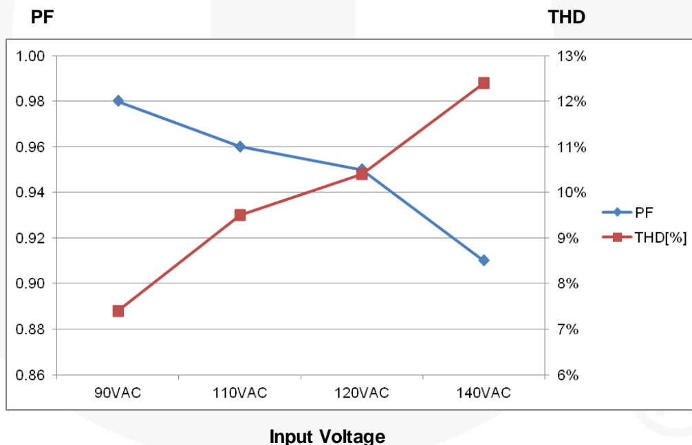
Figure 24. Power Factor & Total Harmonic Distortion (60Hz)
