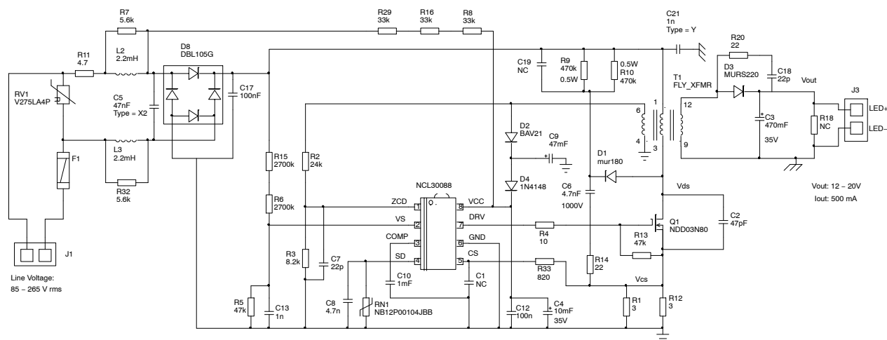
Figure 1. Application Schematic
