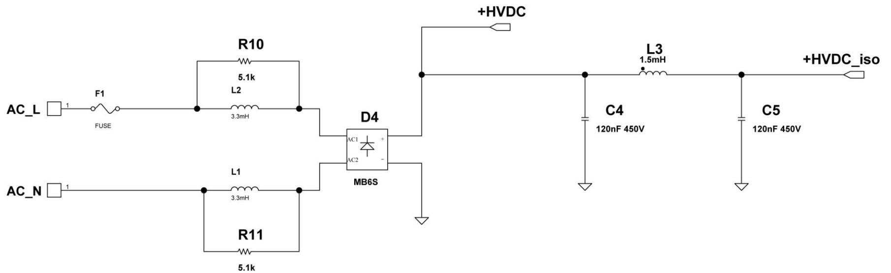
Figure 1: Input Schematic
