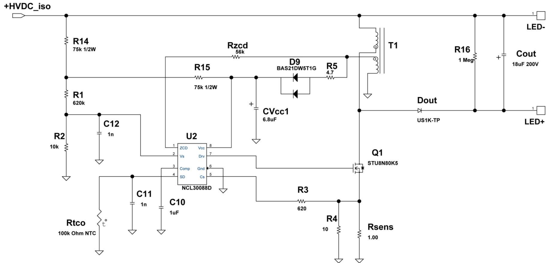
Figure 2: Main Schematic
