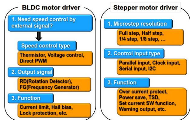
Figure 14. Selecting a BLDC or Stepper Motor Driver
