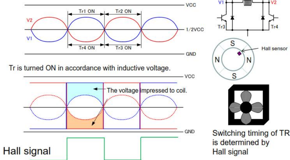
Figure 6. Single-phase BLDC Motor Control
