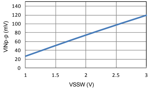
Figure 9 Voltage difference of IN1 and IN2 making Soft-SW width vs SSW voltage
