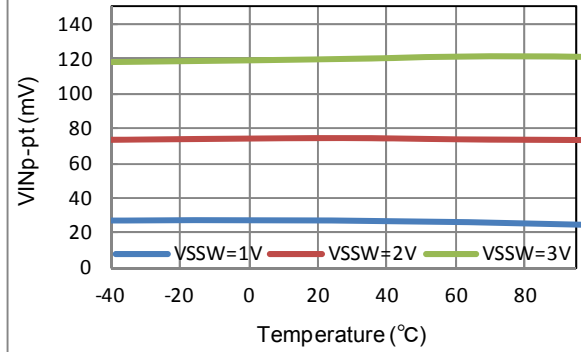
Figure 10 Voltage difference of IN1 and IN2 making Soft-SW width vs Temperature
