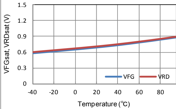
Figure 11 RD/FG output pin low voltage vs Temperature
