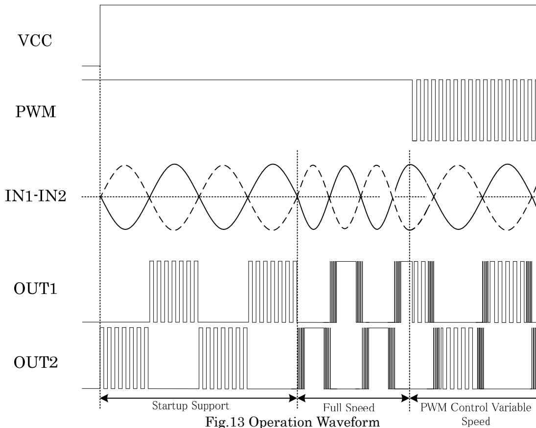
Fig.13 Operation Waveform
