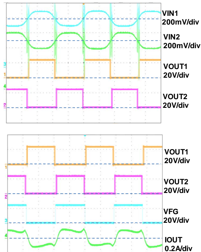
Fig.14 Operation Waveform
