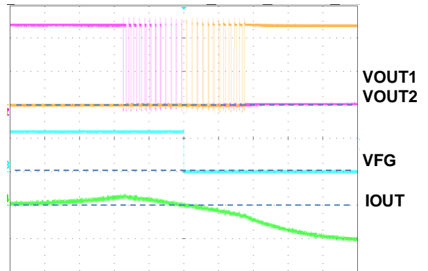
LV8860V Full-Speed 200us/div
