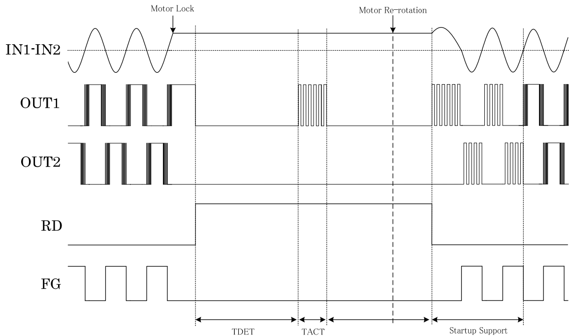
Fig.24 Lock protector operation waveform
