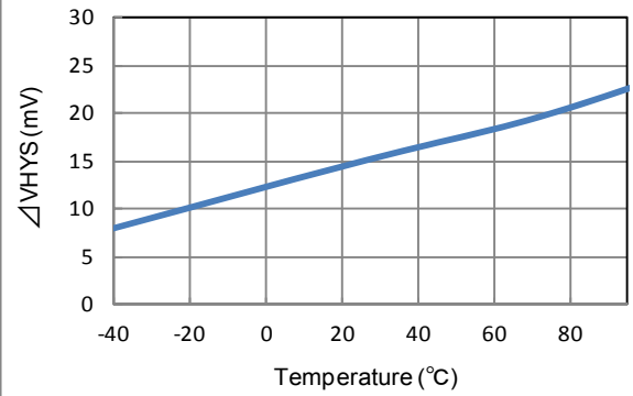
Figure 12 FG comparator hysteresis width vs Temperature
