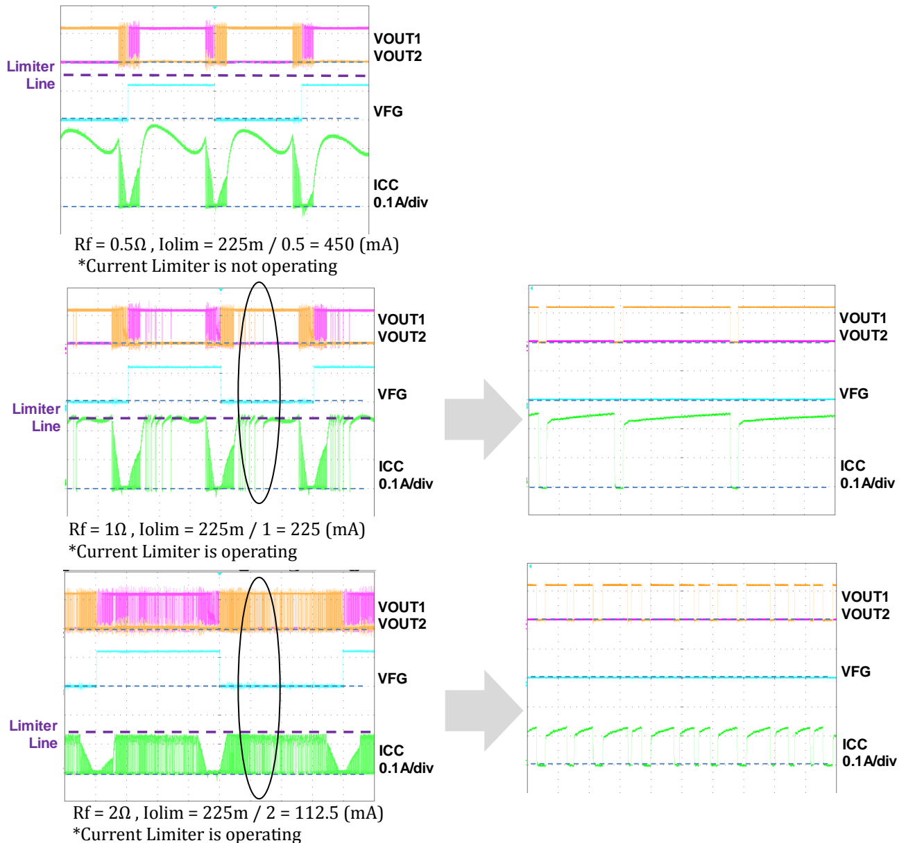
Fig.23 Current Limiter operation waveform
