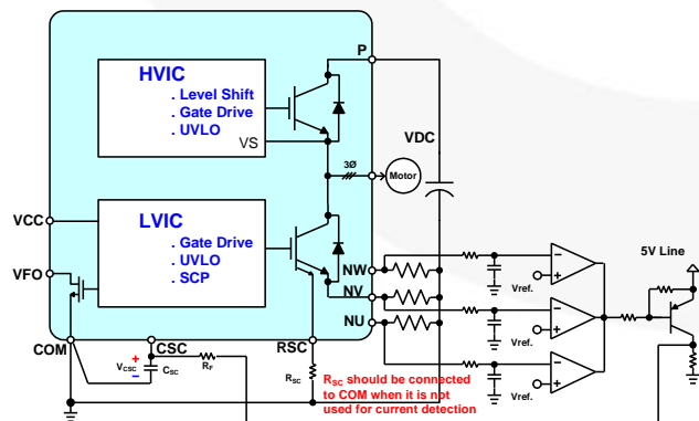
Figure 24. Recommended Circuitry for Over-Current & Short-Circuit Protection without RSC Pin Usage
