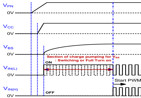
Figure 34. Timing Chart of Initial Bootstrap Charging
