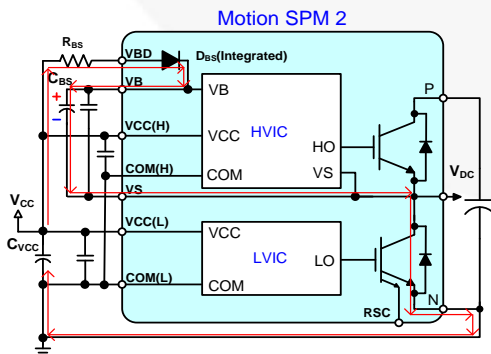
Figure 33. Current Path of Bootstrap Circuit for the Supply Voltage (V BS ) of a HVIC when Low-Side IGBT Turns On
