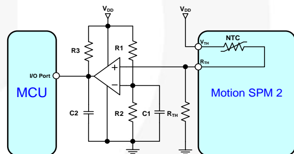
Figure 46. OT Protection Circuit by Comparator
