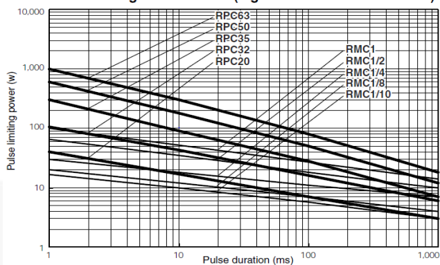
Figure 41. Example of Pulse Power Curve of Resistor (from KAMAYA OHM)
