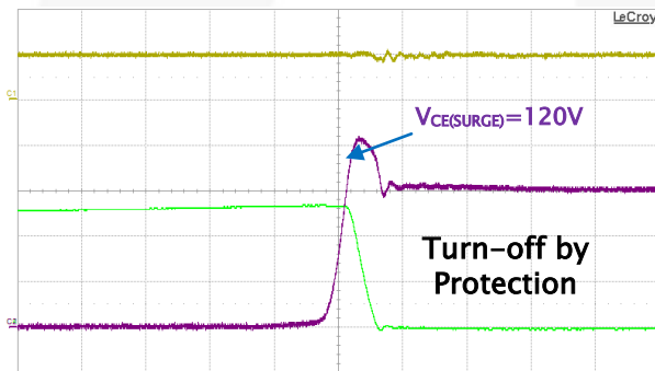
Figure 30. Turn-Off by Soft Off Function (FNA25060, Ref. Condition: V_{DC}=300 V, T_J=25^\circ\text{C} )
