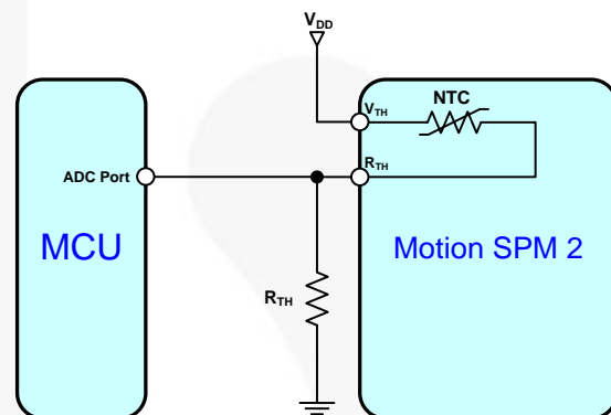
Figure 45. OT Protection Circuit by MCU
