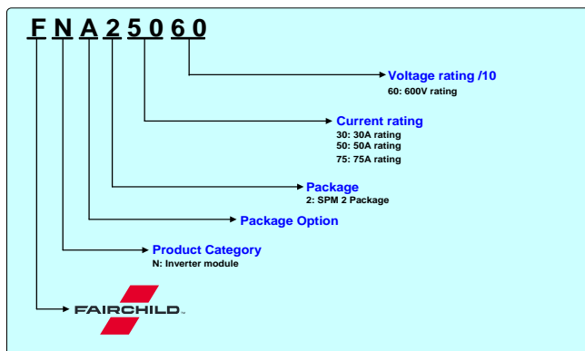
Figure 2. Ordering Information
