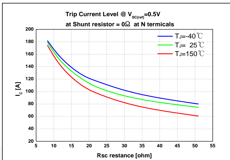
Figure 22. R_{SC} Resistance vs. Trip Current Level for Protection at Variable Junction Temperature of FNA27560
