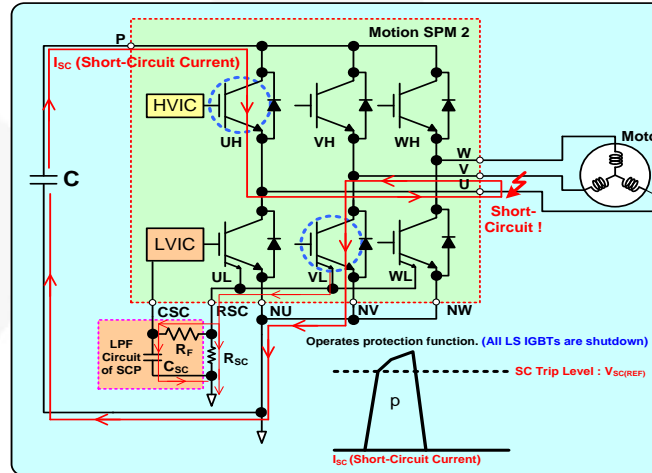
Figure 13. Operation of Short-Circuit Current Protection
