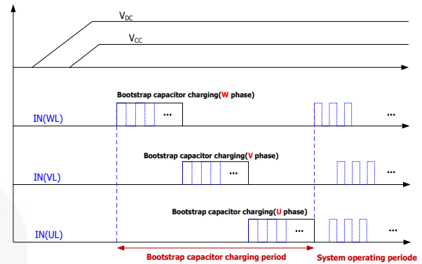
Figure 35. Recommended Initial Bootstrap Capacitors Charging Sequence
