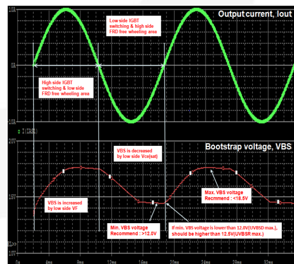
Figure 38. Recommendation of Bootstrap Ripple Voltage during Operation
