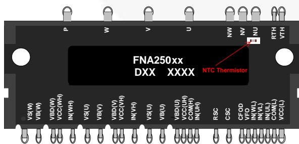
Figure 43. Location of NTC Thermistor in 600-V Motion SPM 2 Series
