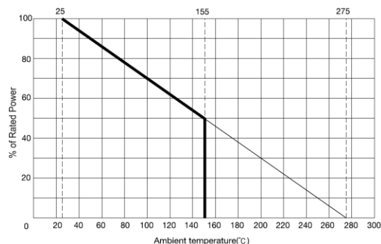
Figure 25. De-rating Curve Example of Shunt Resistor (from RARA Elec.)
