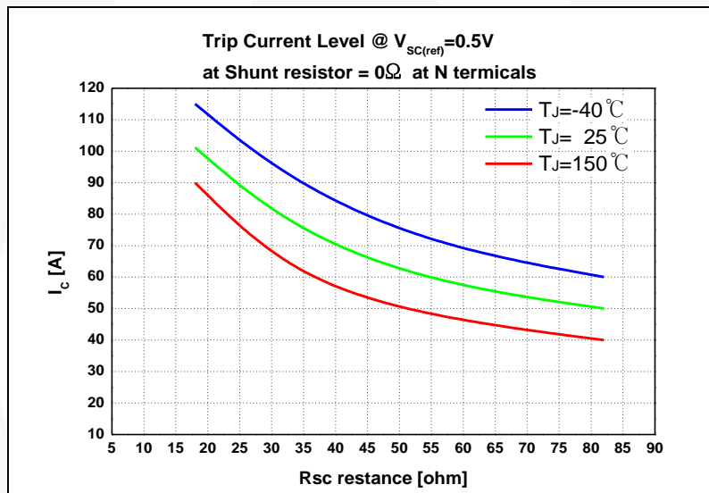
Figure 20. R_{sc} Resistance vs. Trip Current Level for Protection at Variable Junction Temperature of FNA25060
