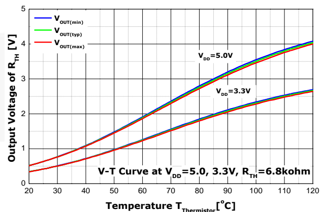
Figure 47. V-T Curve of Figure 45
