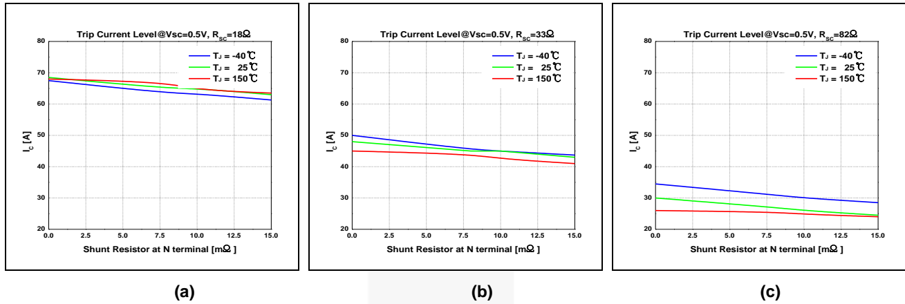
Figure 19. Trip Current Level vs. Shunt Resistor of FNA23060 (a): R_{sc}=18\ \Omega , (b): R_{sc}=33\ \Omega , (c): R_{sc}=82\ \Omega
