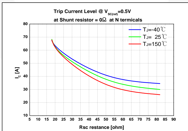
Figure 18. R_{SC} Resistance vs. Trip Current Level for Protection at Variable Junction Temperature of FNA23060
