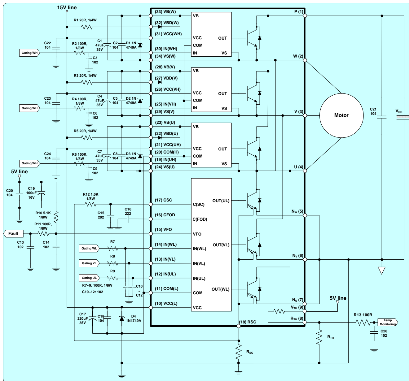
Figure 48. General Application Circuitry for Motion SPM 2 Series
