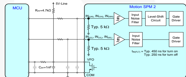
Figure 32. Recommended CPU I/O Interface Circuit
