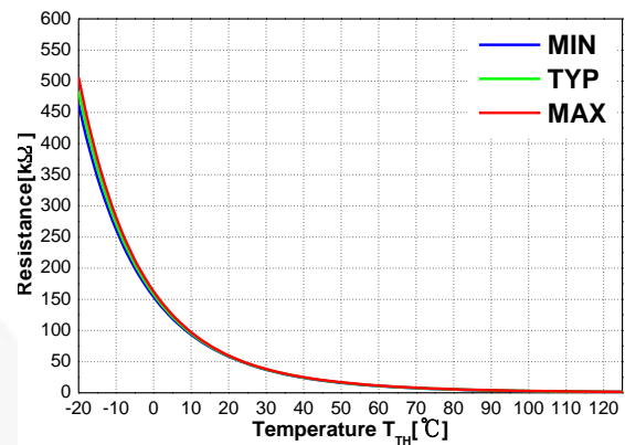
Figure 44. R-T Curve of NTC Thermistor
