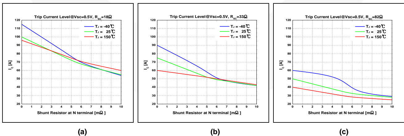
Figure 21. Trip Current Level vs. Shunt Resistor of FNA25060 (a): R_{sc}=18\ \Omega , (b): R_{sc}=33\ \Omega , (c): R_{sc}=82\ \Omega
