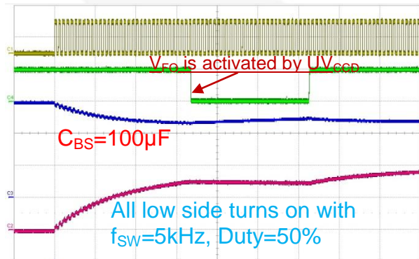
Figure 36. Initial Charging According to Bootstrap Capacitance and Charging Method (Ref. Condition: V_{CC}=15\text{ V}/300\text{ mA} , V_{CC} Capacitor=220 \mu\text{F} , Bootstrap Capacitor=100 \mu\text{F} , R_{BS}=20\ \Omega )
