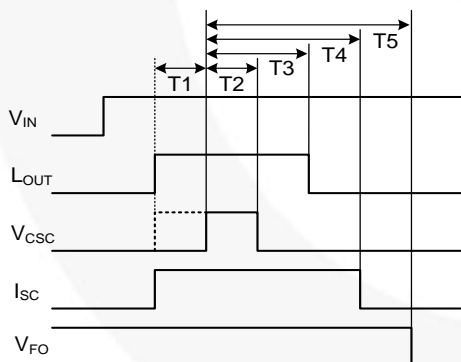
Figure 26. Timing Diagram
