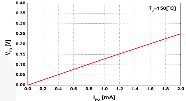
Figure 31. Voltage-Current Characteristics of V_{FO} Terminal
