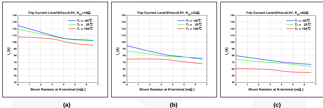
Figure 23. Trip Current Level vs. Shunt Resistor of FNA27560 (a): R_{SC}=18\ \Omega , (b): R_{SC}=33\ \Omega , (c): R_{SC}=82\ \Omega
