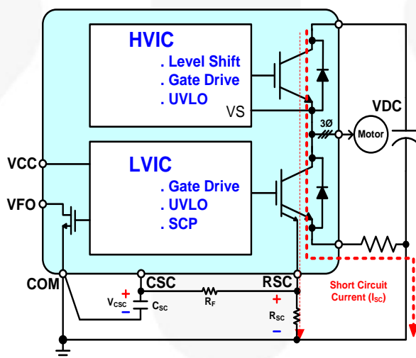
Figure 17. Current Path in Short-Circuit Condition by Leg Short Circuit
