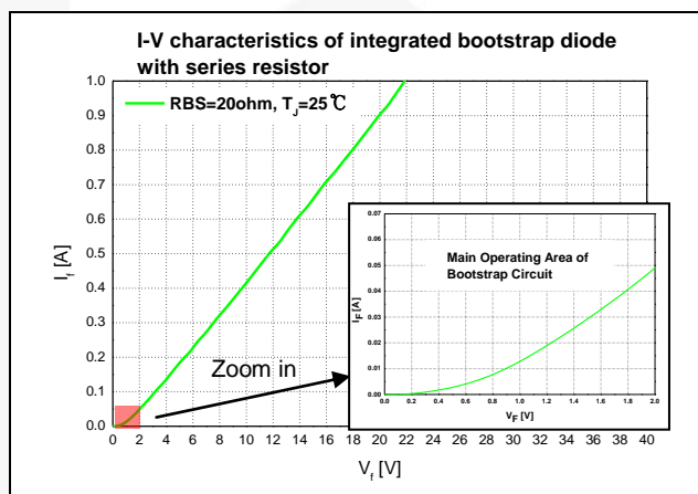
Figure 40. I-V Characteristics of Integrated Bootstrap Diode Series with Series Resistor
