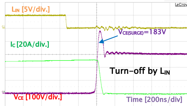
Figure 29. Turn-Off by Input (FNA25060, Ref. Condition: V_{DC}=300 V, T_J=25^\circ\text{C} )
