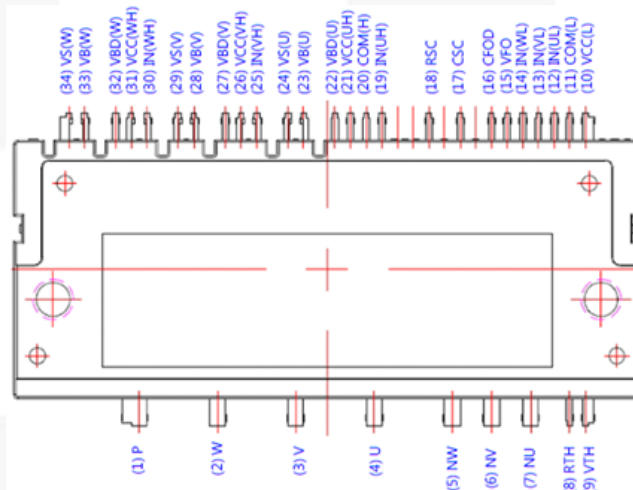
Figure 4. Package Top-View and Pin Assignment
