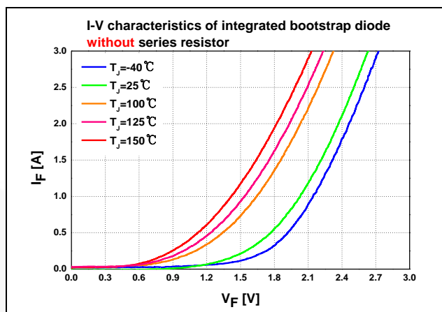
Figure 39. I-V Characteristics of Integrated Bootstrap Diode Series without Series Resistor
