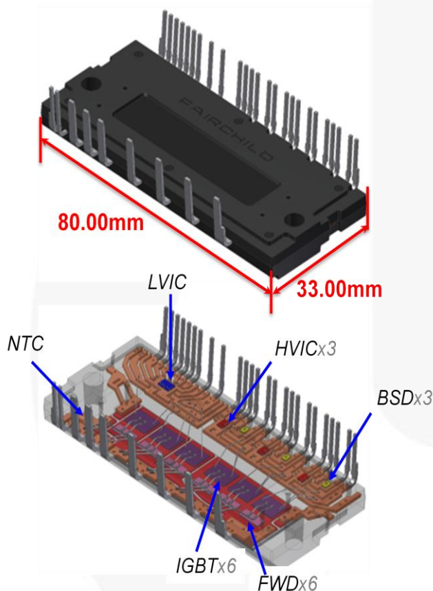
Figure 42. 600-V Motion SPM 2 Series
