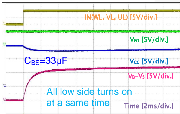
Figure 34. Timing Chart of Initial Bootstrap Charging
