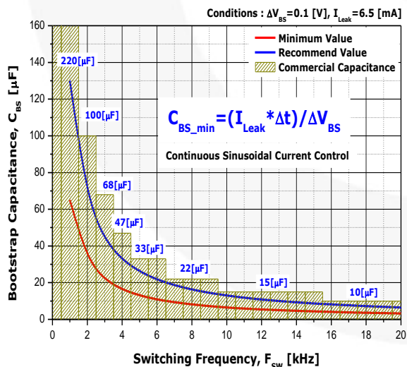
Figure 37. Capacitance of Bootstrap Capacitor on Variation of Switching Frequency
