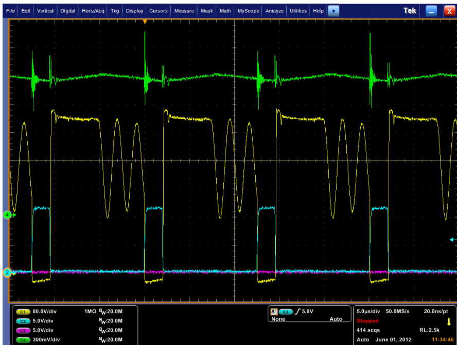
Figure 5. Adjustable PFC Disable
