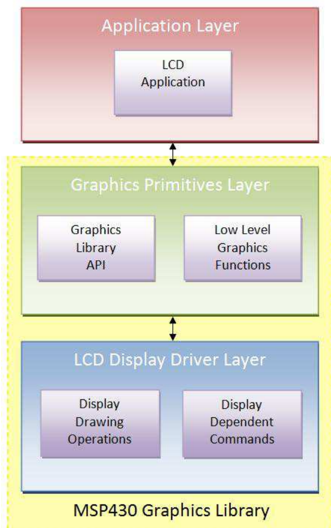
Figure 2. System Overview Stack Diagram
